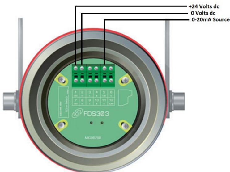
Figure 5: 3 Wire Termination
