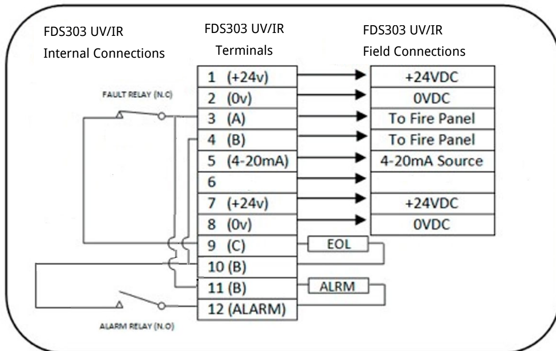
Figure 7: FDS303 UV/IR Internal Inter-connections
